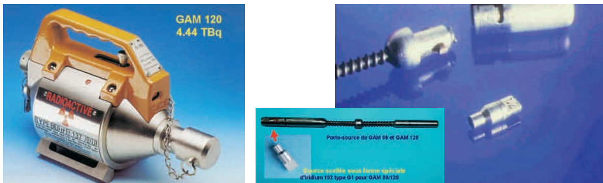
Gammagraphy equipment and its radioactive source
