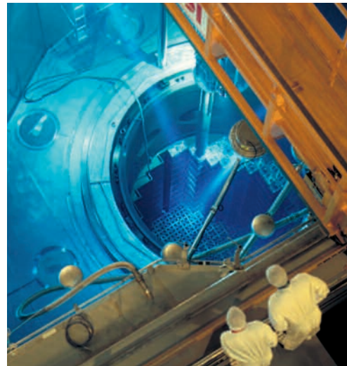
Fuel handling in vessel
